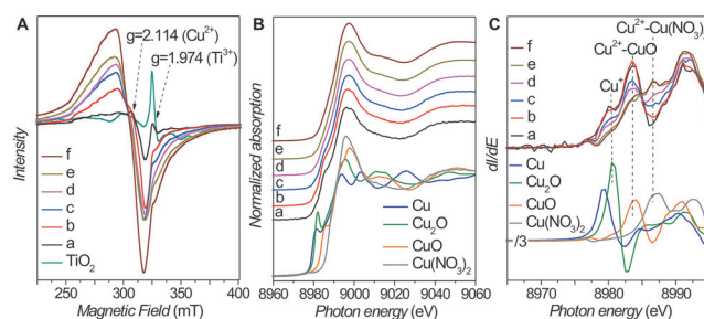
Figure 4. A) EPR spectra, B) Cu K-edge XANES spectra, and C) differentiated Cu K-edge XANES spectra of (a) 0.05 wt-CuO x /TiO 2 , (b) 0.2 wt-CuO x /TiO 2 , (c) 0.5 wt-CuO x /TiO 2 , (d) 1 wt-CuO x /TiO 2 , (e) 2 wt-CuO x /TiO 2 , and (f) 5 wt-CuO x /TiO 2 composites.
