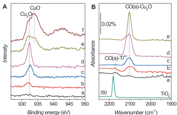
Figure 3. A) Cu 2p 3/2 XPS spectra and B) in-situ DRIFTS spectra of CO adsorption of (a) 0.05 wt-CuO x /TiO 2 , (b) 0.2 wt-CuO x /TiO 2 , (c) 0.5 wt-CuO x /TiO 2 , (d) 1 wt-CuO x /TiO 2 , (e) 2 wt-CuO x /TiO 2 , and (f) 5 wt-CuO x /TiO 2 composites. The in-situ DRIFTS spectrum of CO adsorption on bare TiO 2 nanorods is also included as the comparison.
